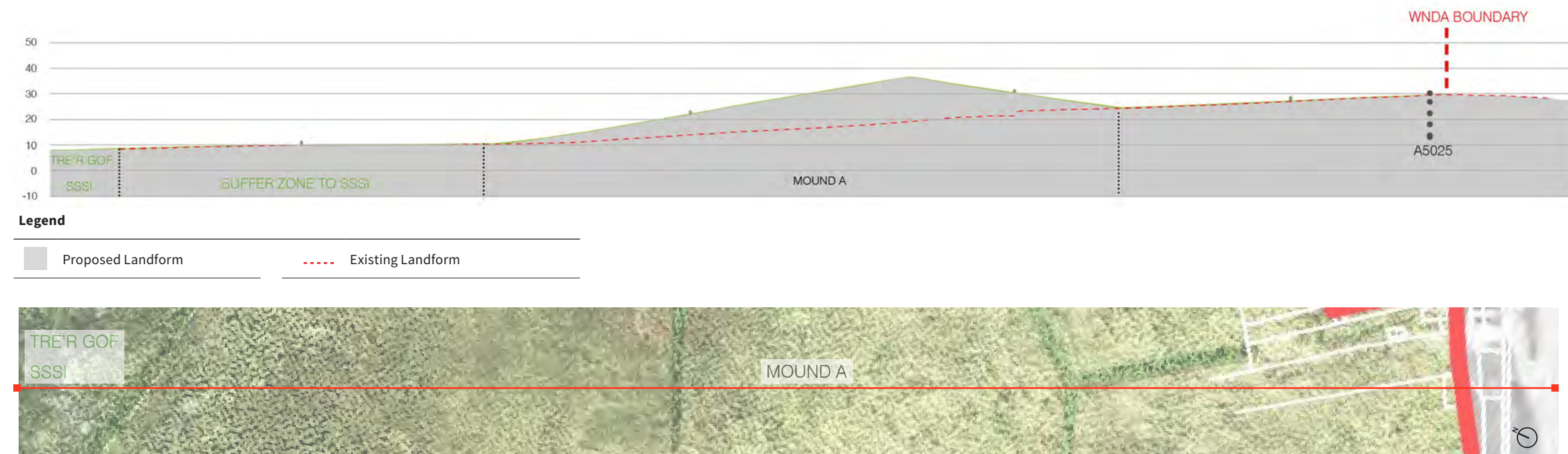
Section 8 : Mound A transversal section
