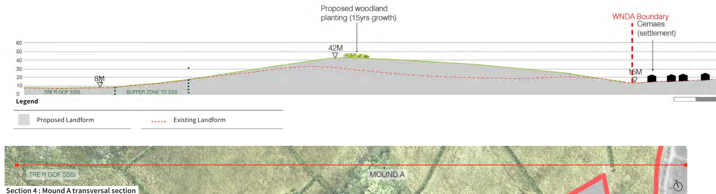
Figure 6-8 Illustrative sections through landform on restoration 2 of 4
