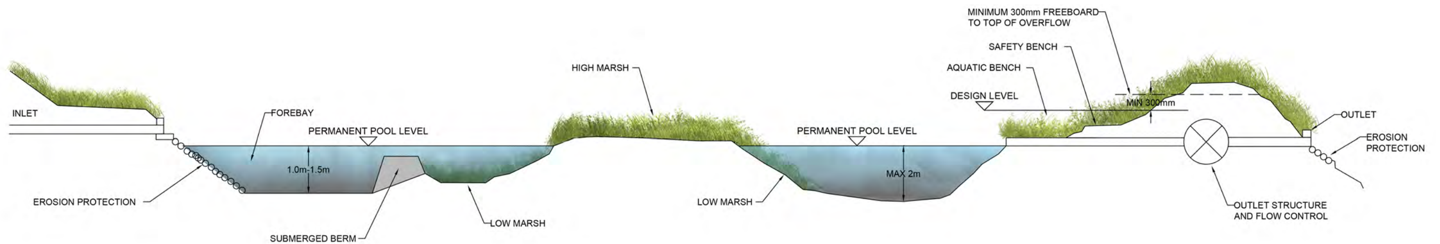
Figure 6-14 b. Typical section of a sedimentation pond
